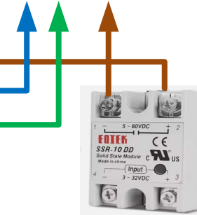
SSR Bed Heater
